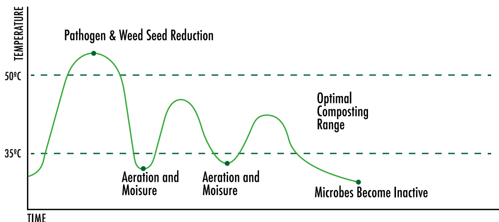
Fig. 5.13 Correct temperature phases for composting
